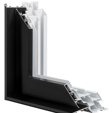
Volet contemporain double Double Contemporary Sash
